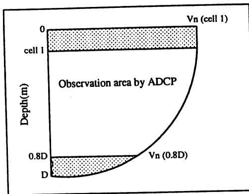
Fig. 6 Assumed current velocity distribution
