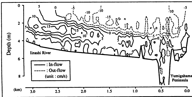
Fig. 4(c) Sectional current velocity distribution around section A during a spring tide at the 8th observation
