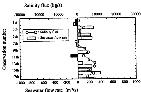
Fig. 7(a) Net seawater and salinity exchange during a neap tide around section A
