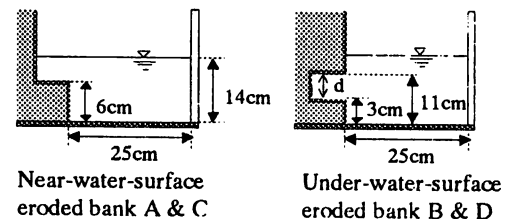
Fig. 2(a) Cross section of 11.5 hours eroded bank
