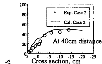
(c) Depth averaged cross sectional velocity distribution
