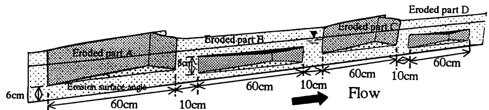
Fig. 2 Side view of 11.5 hours model eroded bank shapes
