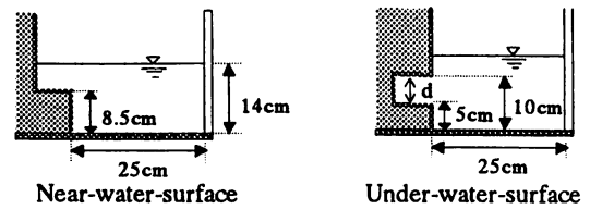
Fig. 1(a) Cross section of 5 hours eroded bank
