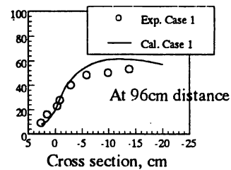
(c) Depth averaged cross sectional velocity distribution
