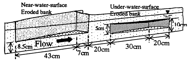
Fig. 1 Side view of 5 hours model eroded bank shapes
